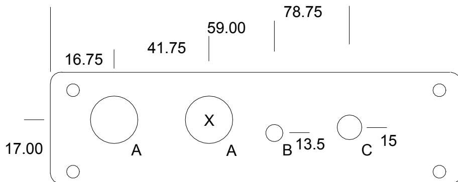
Front panel
