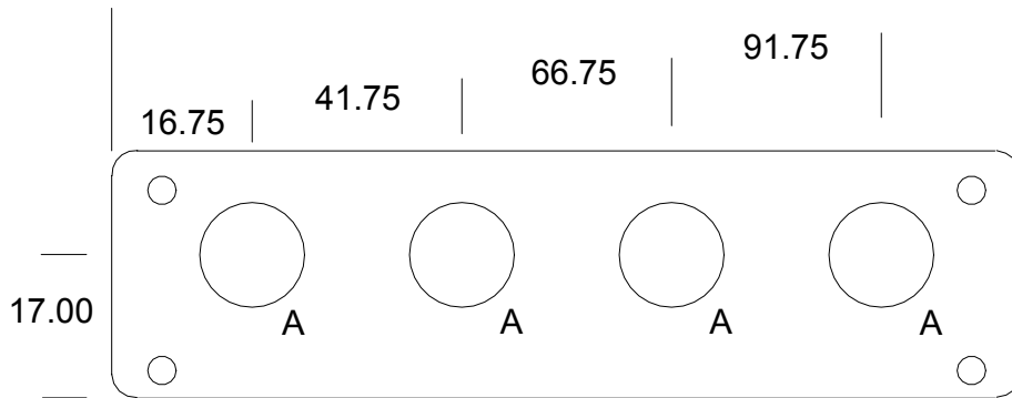
All drillings required for all options Rear panel
