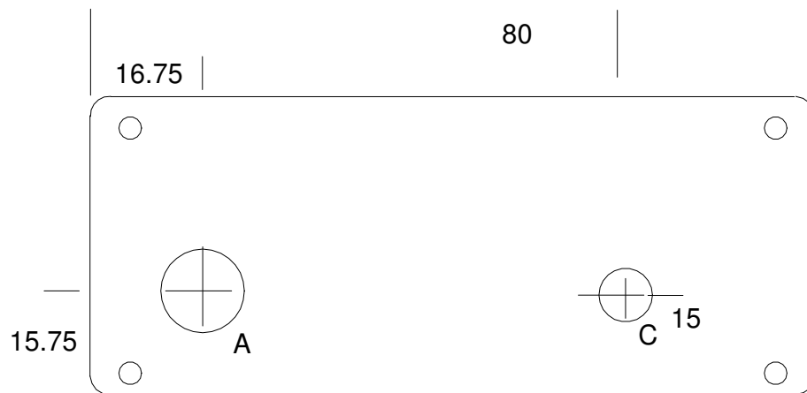
Front panel
