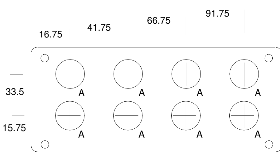
Rear panel
